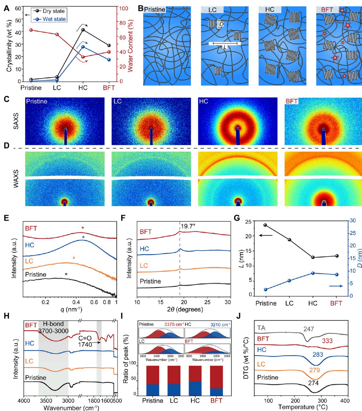
Figure 2. Characterization of hydrogel patches and their structural evolution. (A) Crystallinity and water content comparison of pristine, LC, HC, and BFT patches in dry and wet states. (B) Schematic illustrations showing the microstructural differences between pristine, LC, HC, and BFT patches, highlighting the formation of nanocrystalline domains and TA-mediated hydrogen bonds in BFT patches. (C) Small-angle X-ray scattering (SAXS) patterns showing the nanostructure of different patches. (D) Wide-angle X-ray scattering (WAXS) patterns demonstrating the crystalline structures in various patches. (E) SAXS intensity profiles indicating the structural changes in different patches. (F) WAXS intensity profiles showing the diffraction peak at 19.7° associated with crystalline domains. (G) Distance between crystalline domains ( L ) and Crystalline domain size ( D ) calculated from SAXS and WAXS data. (H) ATR-FTIR spectra displaying the hydrogen bond and C=O stretching regions, illustrating the differences in chemical bonding among the patches. (I) Ratio of FTIR peak intensities highlighting the differences in hydrogen bond strength and content across the patches. (J) Differential thermogravimetric (DTG) analysis showing the thermal stability and decomposition temperatures of different patches, with BFT patches exhibiting the highest thermal stability due to dual cross-linking.
