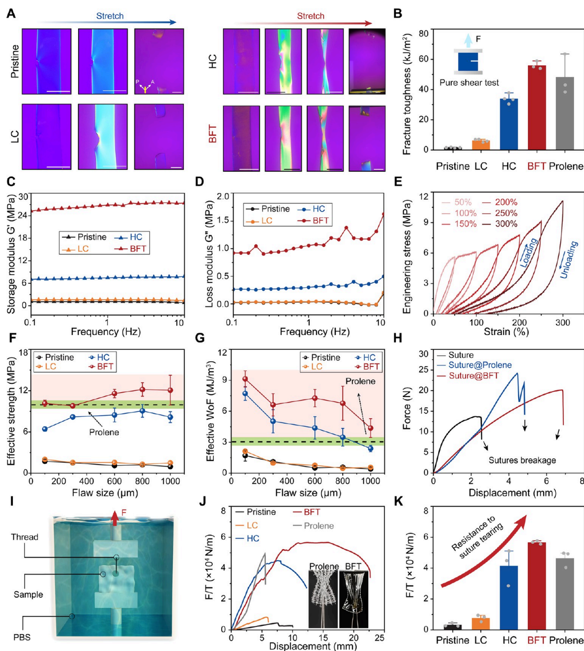
Figure 3. Mechanical properties and flaw tolerance of hydrogel patches. (A) Representative polarized optical images showing the birefringence of pristine, LC, HC, and BFT patches under uniaxial stretching. Three independent experiments were conducted with similar results. Scale bars: 5 mm. (B) Fracture toughness of pristine, LC, HC, BFT, and Prolene patches, measured by pure shear tests, demonstrating the superior toughness of BFT patches. (C–D) Dynamic mechanical analysis (DMA) showing the storage modulus ( G' ) and loss modulus ( G'' ) of pristine, LC, HC, and BFT patches as a function of frequency, highlighting the mechanical stability of BFT patches under different loading conditions. (E) Engineering stress–strain curves during cyclic loading and unloading. (F–G) Residual strength and work of fracture of patches with varying flaw sizes, comparing the flaw tolerance of BFT patches with other samples and the Prolene mesh patch. (H) Force–displacement curves for suture tear resistance tests, comparing BFT and Prolene patches in sutured configurations. (I) Schematic of the setup for suture tear resistance tests in a PBS environment, replicating physiological conditions. (J) Force/tear displacement curves of sutured patches. (K) Bar graph summarizing the suture tear resistance ( F/T ) of the different patches.
