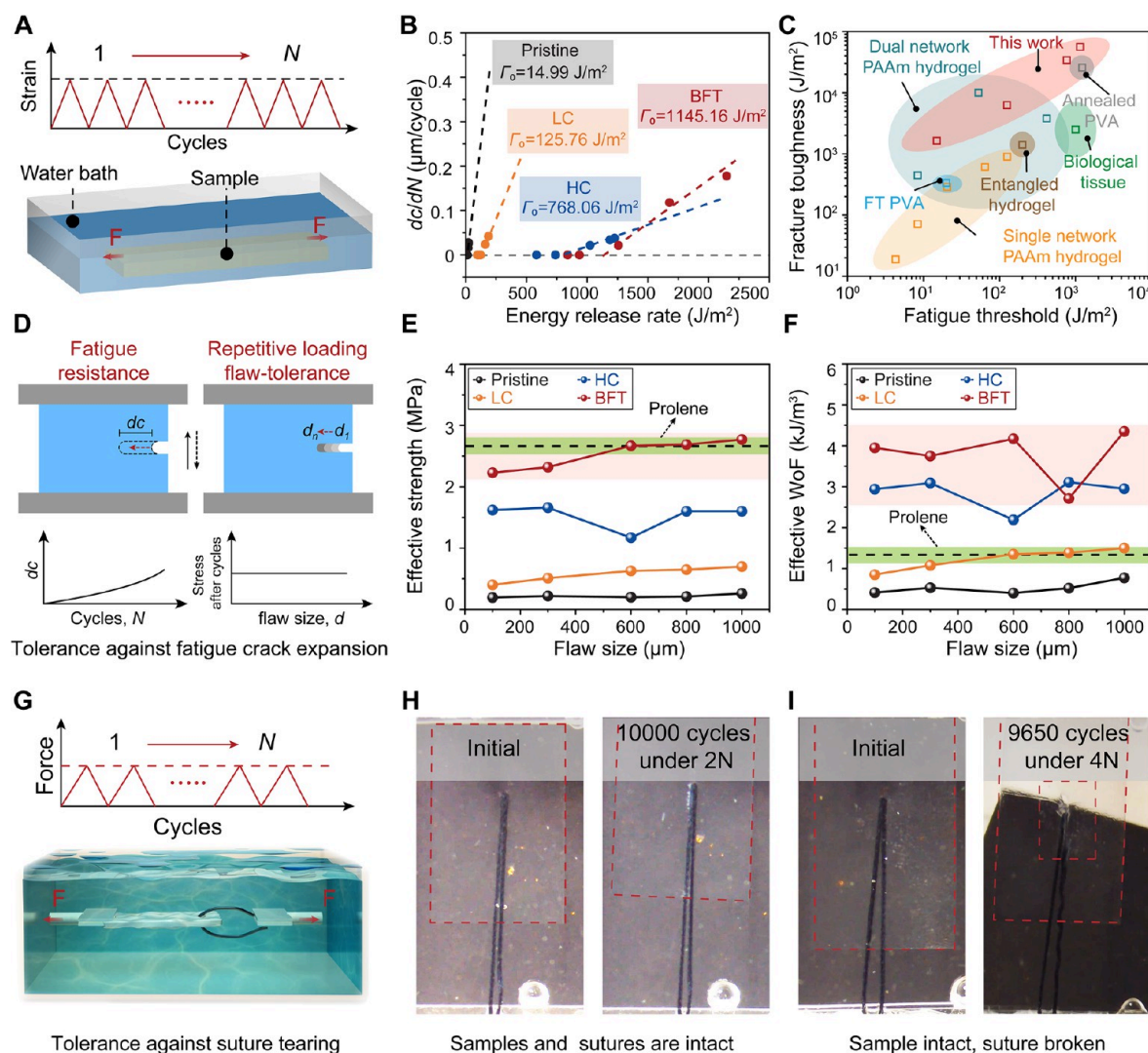
Figure 4. Fatigue resistance and flaw-tolerance of patches. (A) Schematic of cyclic loading test setup for evaluating fatigue threshold. (B) Plot of crack growth rate per cycle ( dc/dN ) as a function of energy release rate ( G ) for different patch groups: pristine, LC, HC, and BFT. (C) Ashby plot comparing fracture toughness and fatigue threshold among various hydrogel systems. (D) Illustration of the difference between fatigue resistance test and flaw-tolerance test under repetitive loading, emphasizing the tolerance against fatigue when samples with crack. (E–F) Residual strength and work of fracture versus flaw size for different patches after 5000 cycles under 50% strain, including a commercial Prolene patch. (G) Schematic of cyclic loading test setup for evaluating fatigue resistance to suture tearing. (H–I) Photographs showing the integrity of samples and sutures before and after cyclic loading under 2N and 4N loading.
